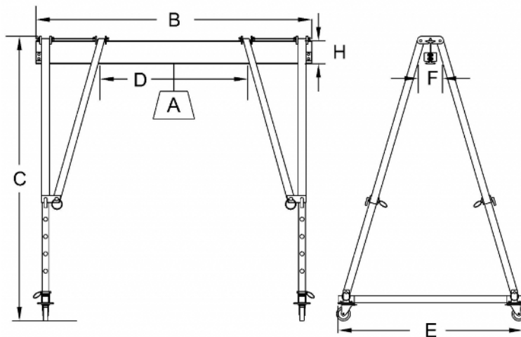
Mighty Mite Dimensional Sketch (Casters Optional) - Click to enlarge
