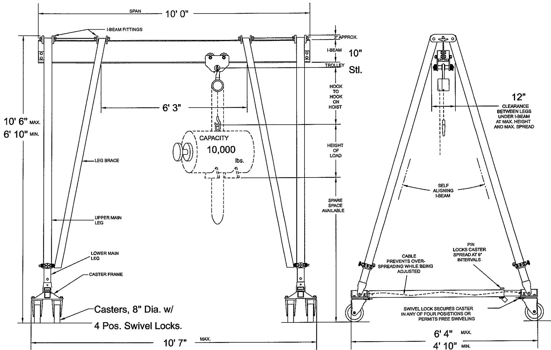
Steel Frames and I-Beam Listed Dimensions are \pm \frac{1}{2} "
