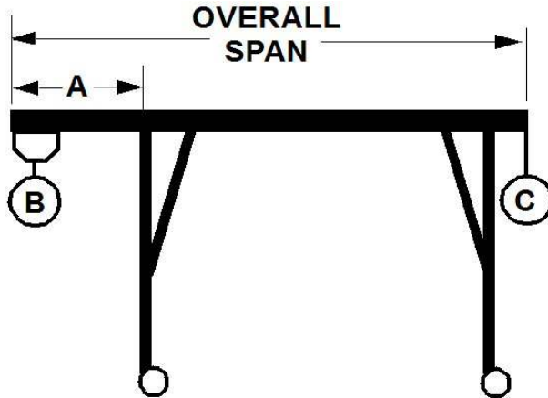
REQUIRED COUNTERWEIGHT AT [C]
